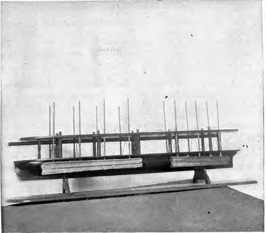
MODEL OF ABRAHAM LINCOLN'S DEVICE FOR LIFTING VESSELS OVER SHOALS.
